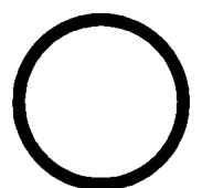
Mercury
