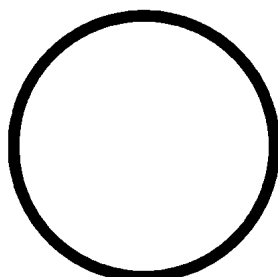
Neptune
