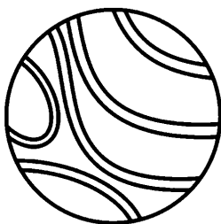
NEPTUNE
